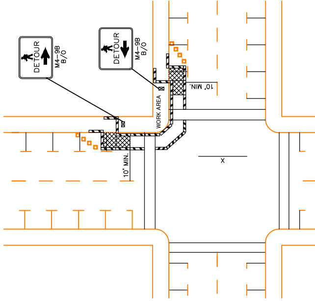
SIDEWALK DIVERSION
