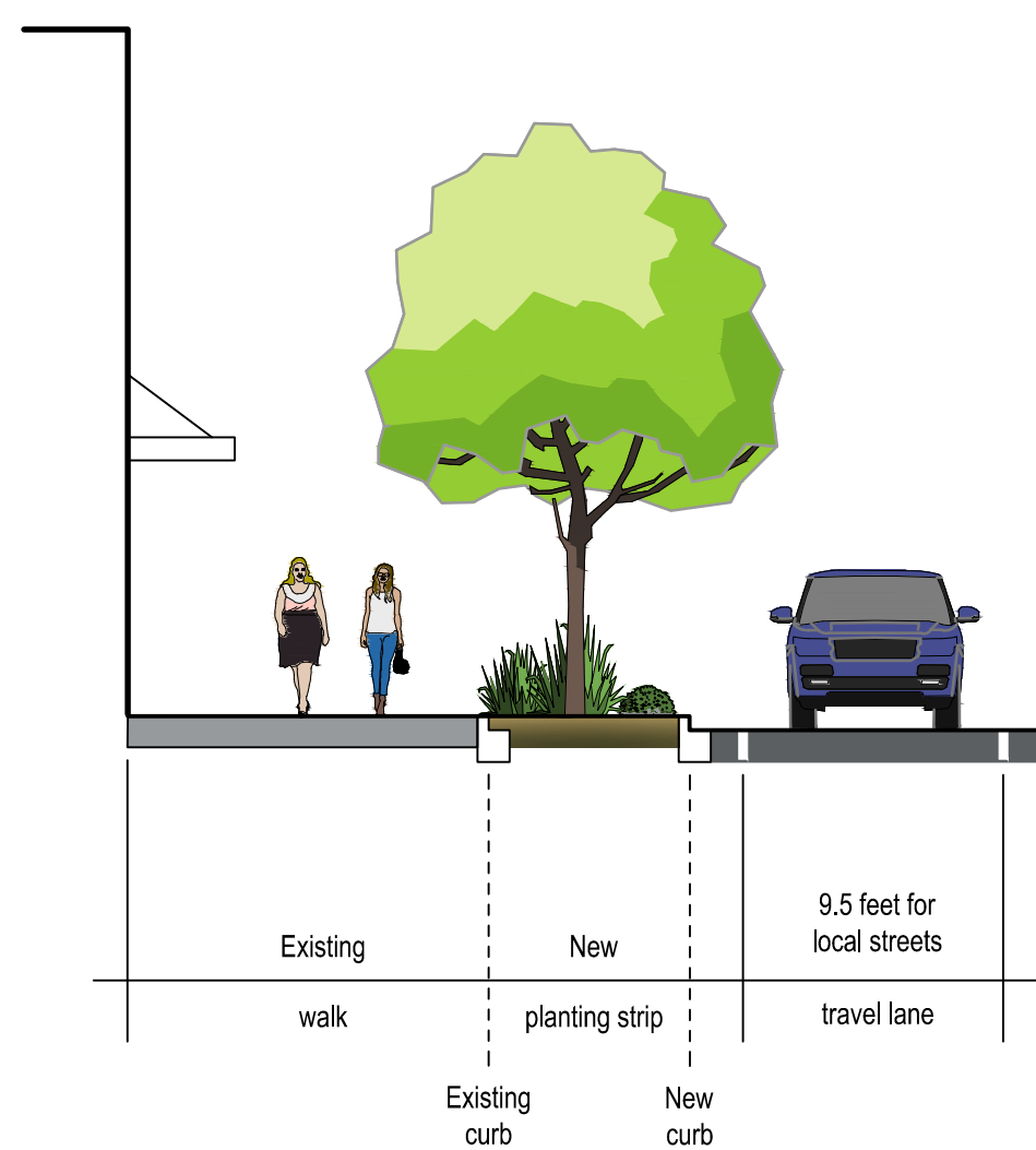
Section/Elevation B-B'
