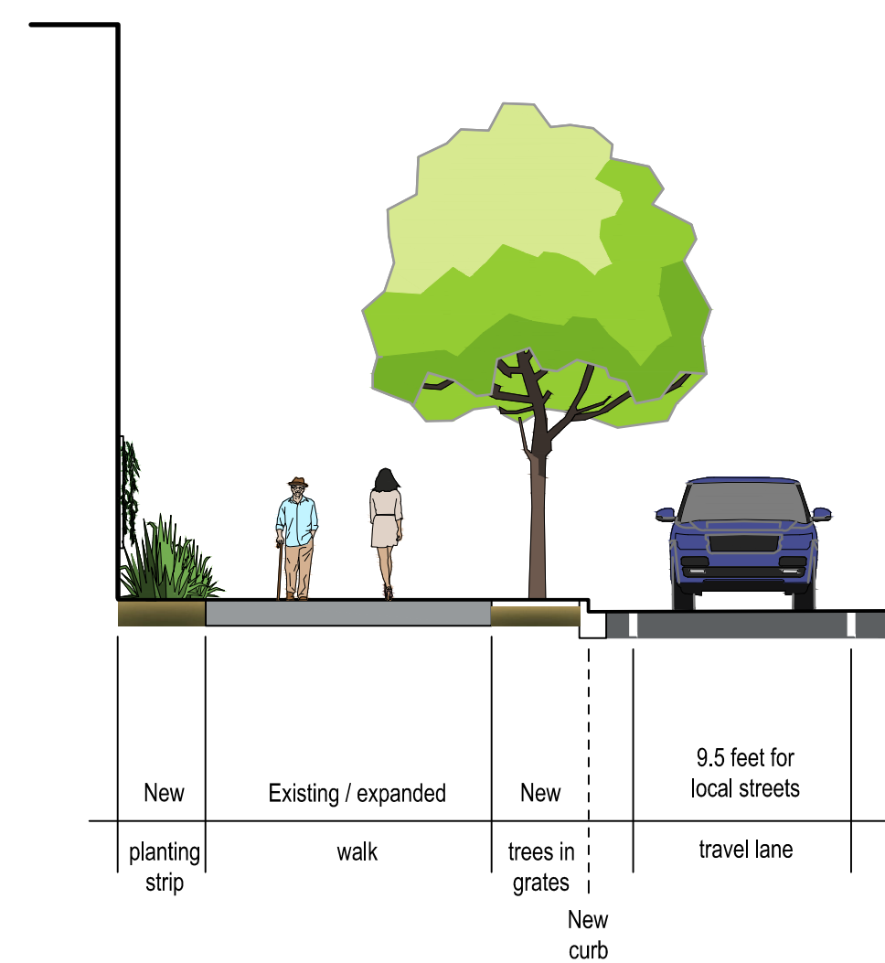
Section/Elevation C-C'
