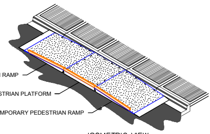
ISOMETRIC VIEW DUAL RAMP
